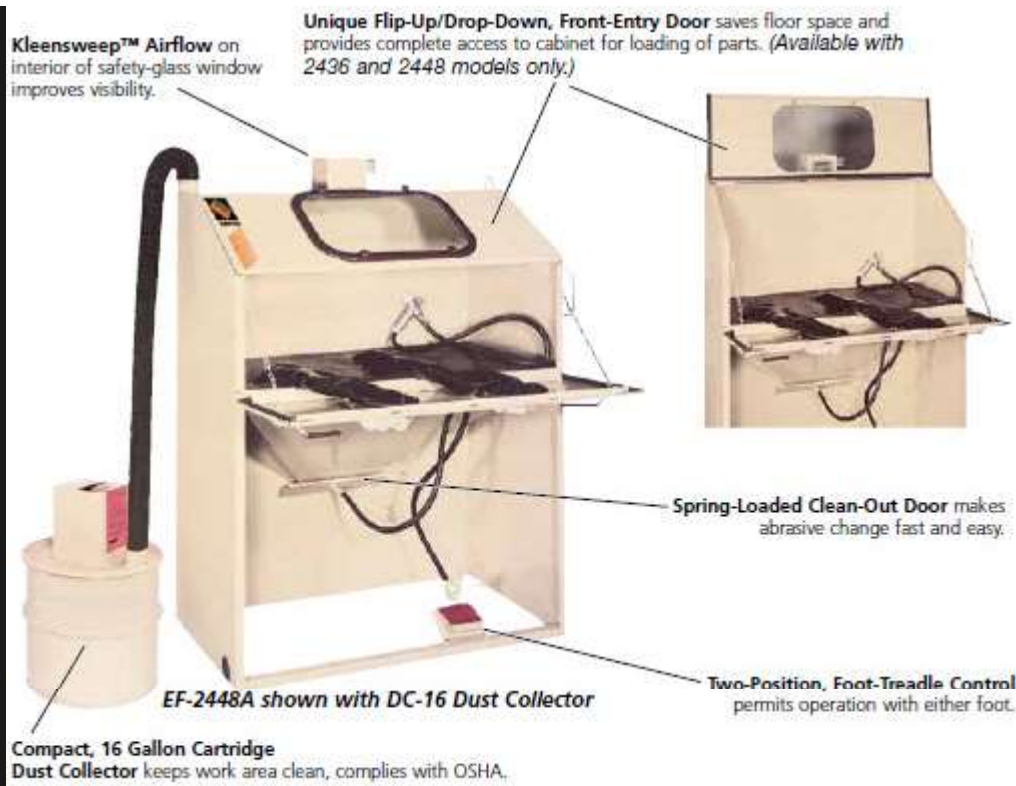
Econo-Finish-Blast-Cabinet-Features
